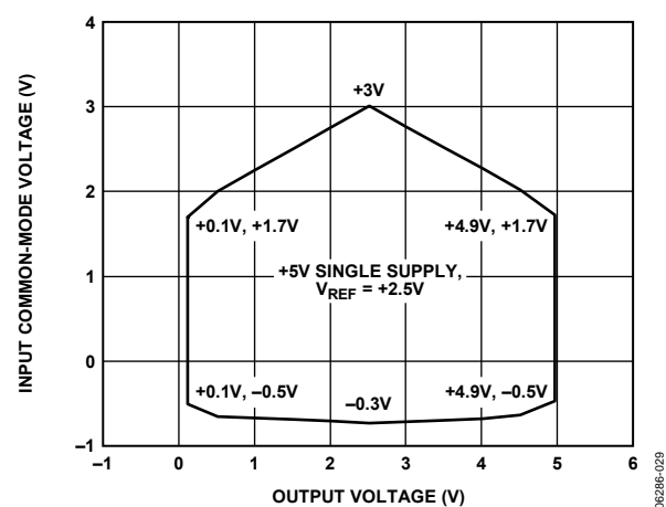
Figure 27. Input Common-Mode Voltage Range vs. Output Voltage, G = 100 , V_S = 5V , V_{REF} = 2.5V
