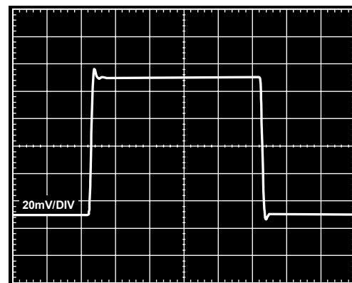
Figure 43. Small Signal Pulse Response, G = 10 , R_{LOAD} = 2\text{ k}\Omega , C_{LOAD} = 100\text{ pF} , V_S = \pm 15\text{ V} , V_{REF} = 0\text{ V}
