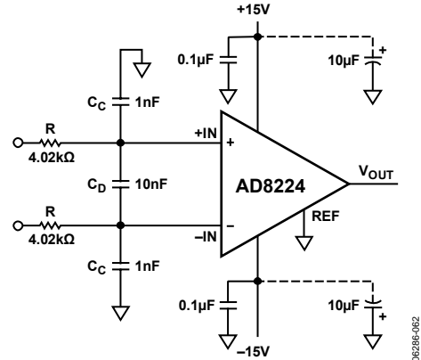
Figure 60. RFI Suppression
