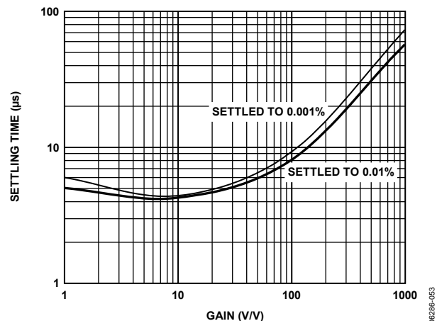
Figure 51. Settling Time vs. Gain for a 10\text{ V} Step, V_S = \pm 15\text{ V} , V_{REF} = 0\text{ V}
