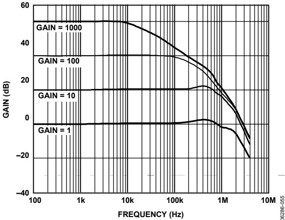
Figure 53. Differential Output Configuration: Gain vs. Frequency
