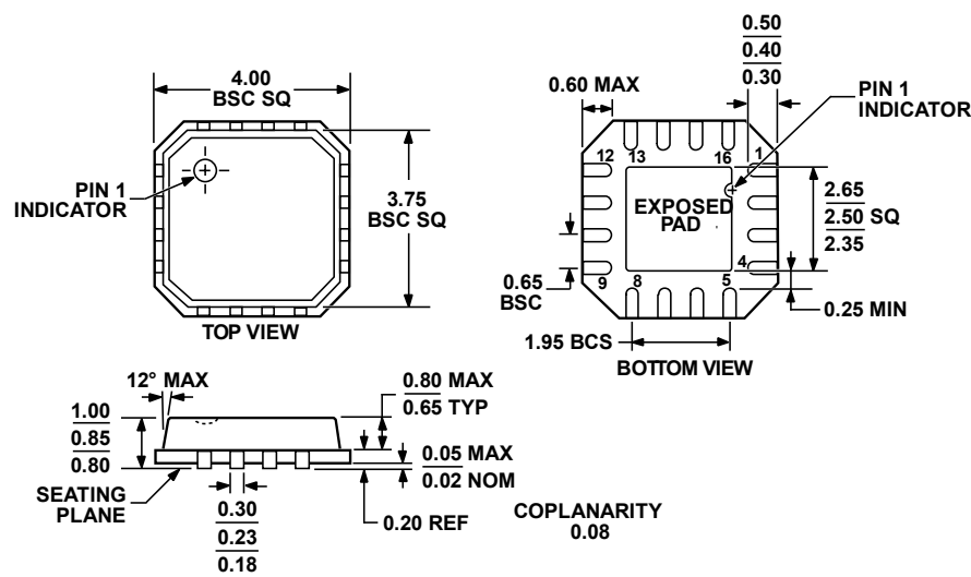
Figure 66. 16-Lead Lead Frame Chip Scale Package [LFCSP_VQ] 4 mm x 4 mm Body, Very Thin Quad (CP-16-13) Dimensions are shown in millimeters
