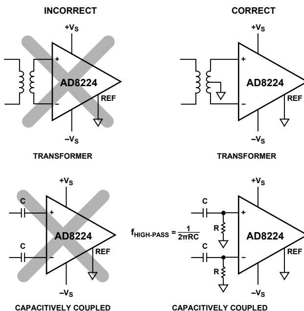
Figure 58. Creating an I_{BIAS} Path
