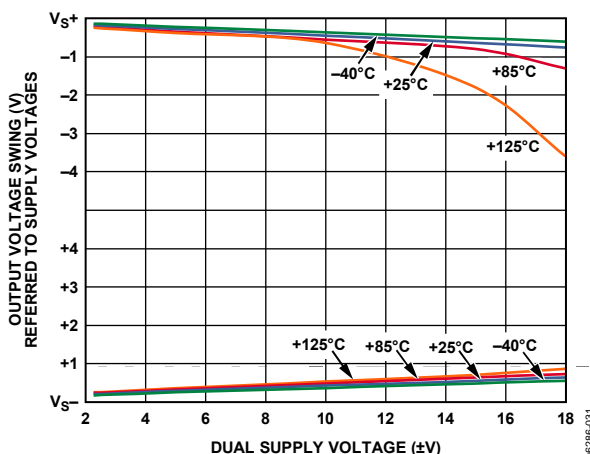
Figure 29. Output Voltage Swing vs. Dual Supply Voltage, R_{LOAD} = 2 kΩ, G = 10 , V_{REF} = 0 V
