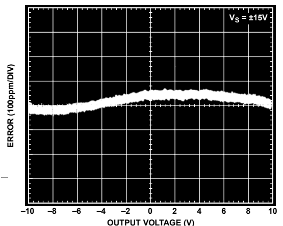
Figure 25. Gain Nonlinearity, G = 1000 , R_L = 10 k\Omega
