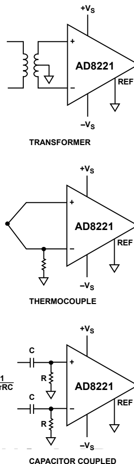
Figure 47. Creating an I BIAS Path
