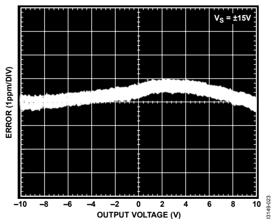
Figure 23. Gain Nonlinearity, G = 1 , R_L = 10 k\Omega
