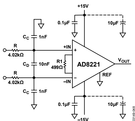
Figure 48. RFI Suppression
