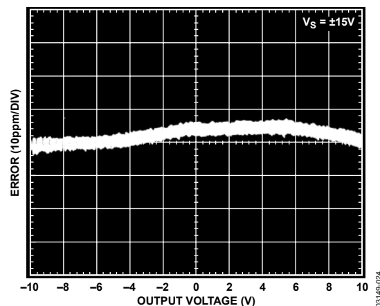
Figure 24. Gain Nonlinearity, G = 100 , R_L = 10 k\Omega
