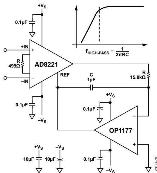
Figure 51. AC-Coupled Circuit
