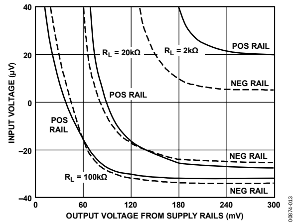
Figure 13. Input Effort Voltage with Output Voltage Within 300 mV of Either Supply Rail for Various Resistive Loads; V_S = \pm 5\text{ V}
