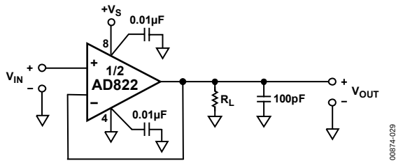
Figure 29. Unity Gain Follower
