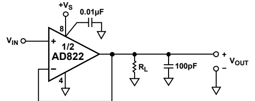
Figure 35. Unity Gain Follower
