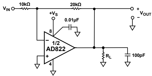
Figure 36. Gain-of-2 Inverter
