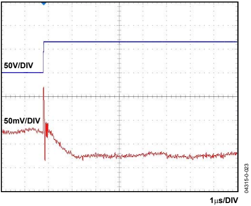
Figure 12. Common-Mode Response
