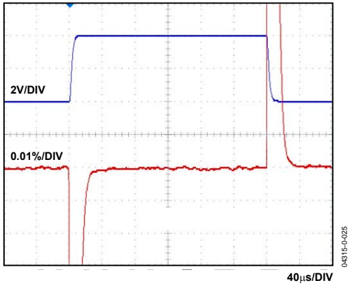
Figure 11. Settling Time
