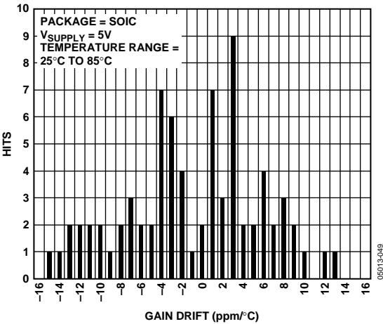
Figure 38. Gain Drift Distribution, SOIC, Temperature Range = 25°C to 85°C
