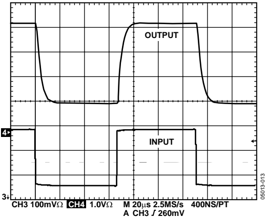
Figure 13. Pulse Response
