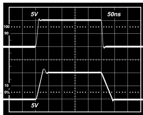
Figure 23. Noninverting Large Signal Pulse Response, R_L = 1k\Omega
