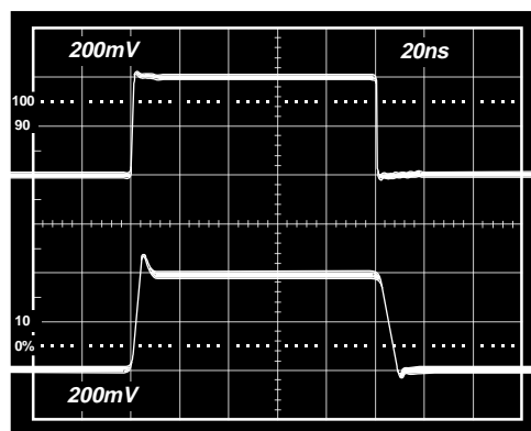
Figure 24. Noninverting Small Signal Pulse Response, R_L = 1k\Omega
