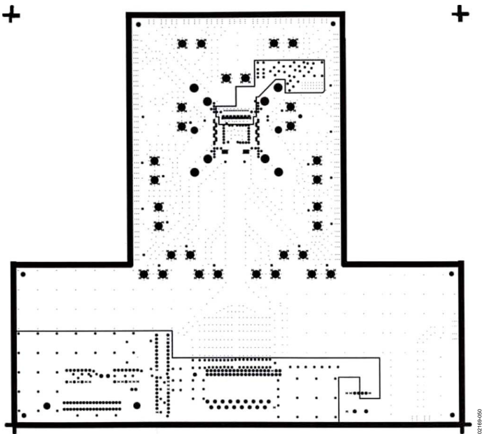
Figure 50. INT2 (Vcc)
