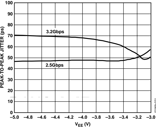
Figure 21. Jitter vs. Supply, PRBS 23
