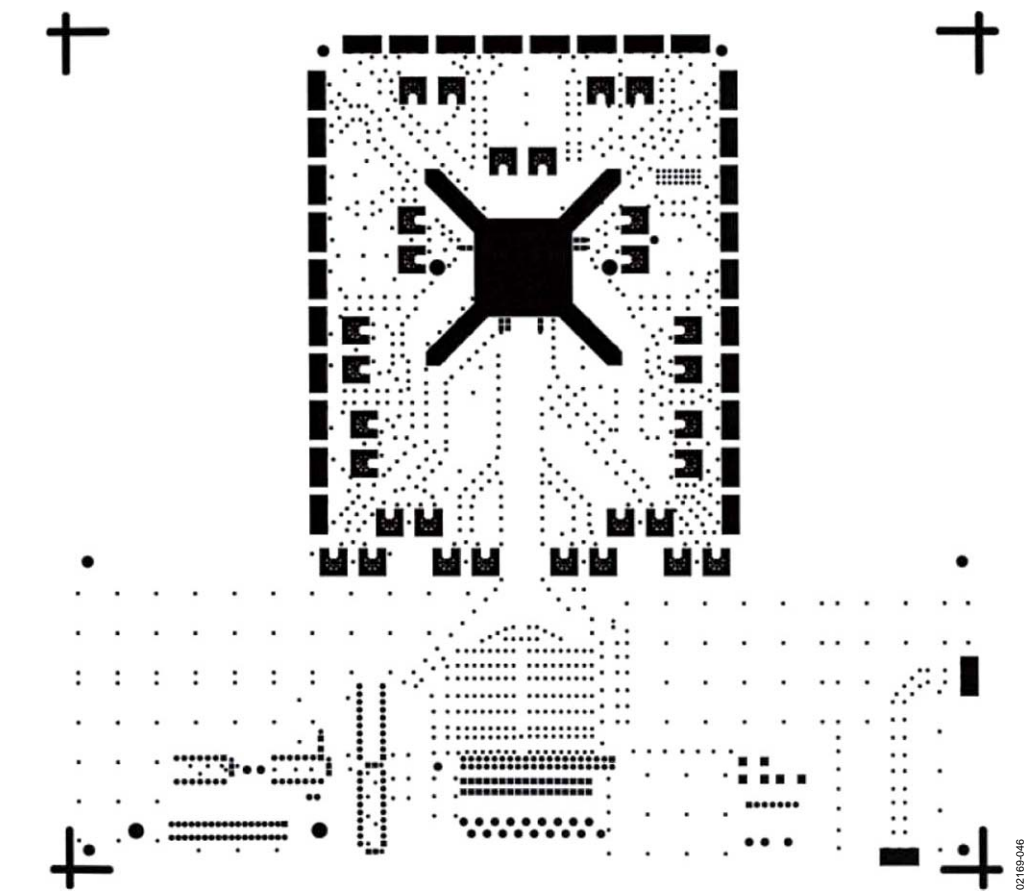
Figure 46. Solder Mask Top
