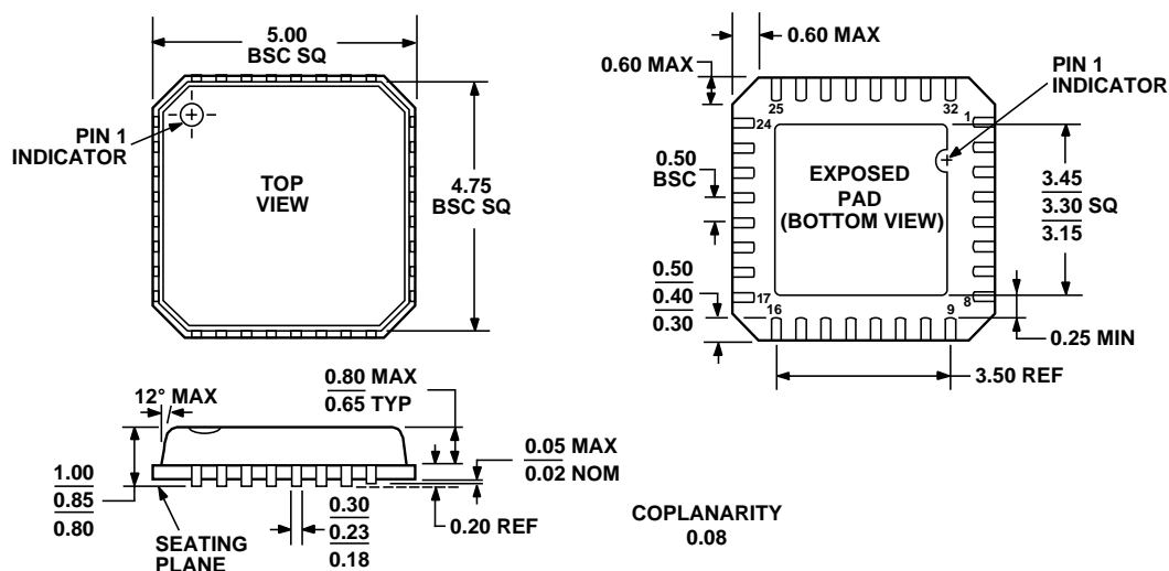
Figure 49. 32-Lead Lead Frame Chip Scale Package [LFCSP_VQ] 5 mm × 5 mm Body, Very Thin Quad (CP-32-3)
