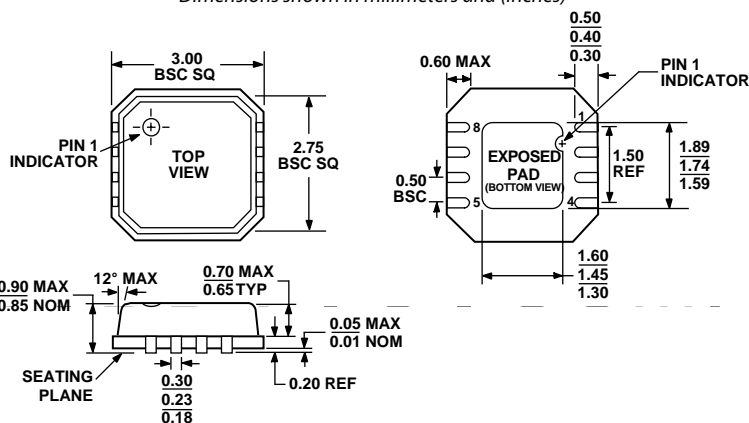
Figure 71. 8-Lead Lead Frame Chip Scale Package [LFCSP_VD] 3 mm x 3 mm Body, Very Thin, Dual Lead (CP-8-2)
