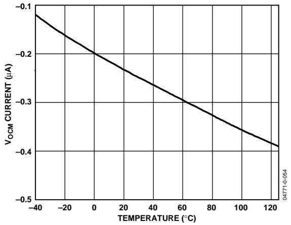
Figure 54. V_{OCM} Bias Current vs. Temperature
