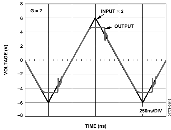
Figure 37. Overdrive Recovery
