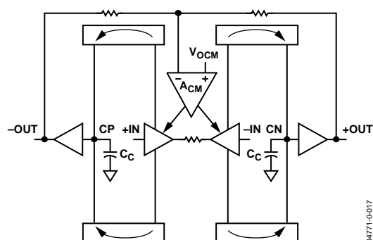
Figure 61. Block Diagram
