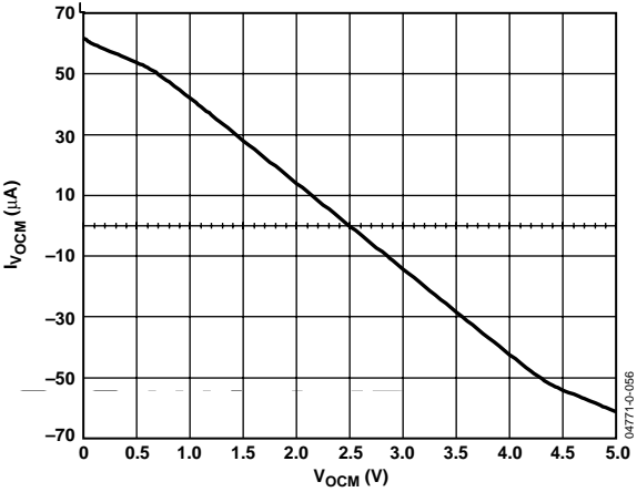
Figure 53. V_{OCM} Bias Current vs. V_{OCM} Input Voltage
