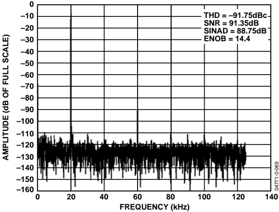
Figure 69. AD8137 Performance on +6 V, -1 V Supplies, -0.45 dBFS
