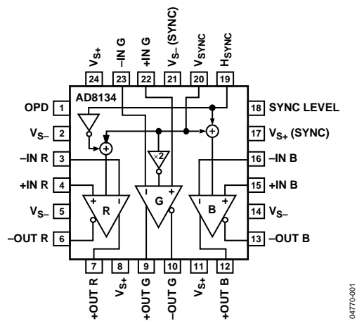
Figure 4. 24-Lead LFCSP
