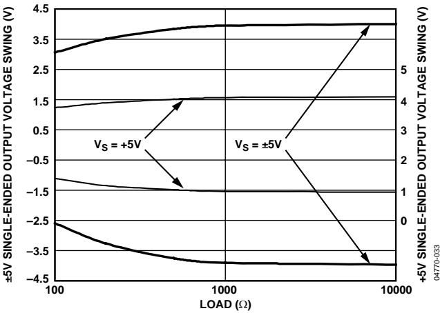
Figure 27. Output Saturation Voltage vs. Output Load
