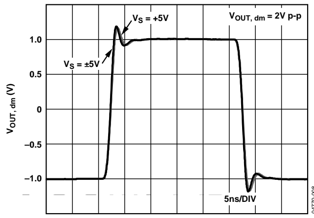
Figure 16. Large Signal Transient Response for Various Power Supply Voltages
