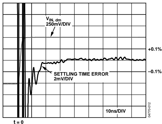
Figure 17. Settling Time (0.1%)
