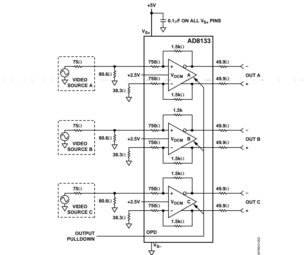
Figure 36. AD8133 in Single-Ended-to-Differential Application
