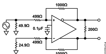
Figure 57. Basic Test Circuit, G = 2
