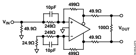
Figure 75. Frequency Boost Circuit
