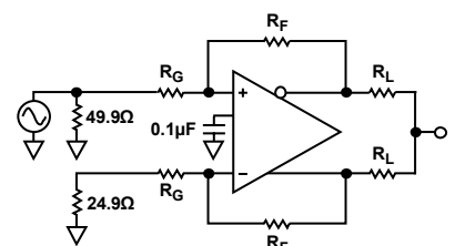
Figure 59. Test Circuit for Output Balance
