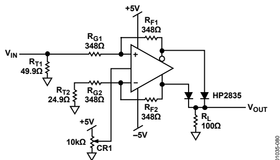
Figure 82. Full-Wave Rectifier
