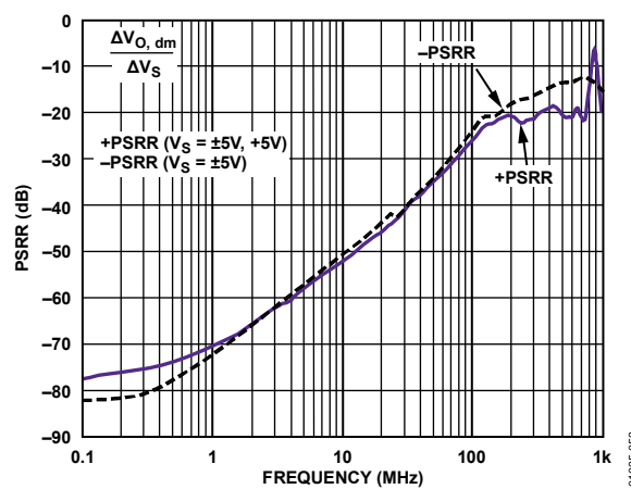
Figure 46. PSRR vs. Frequency
