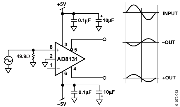
Figure 43. Unity Gain, Single-Ended-to-Differential Amplifier
