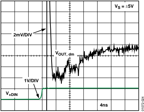
Figure 25. 0.1% Settling Time
