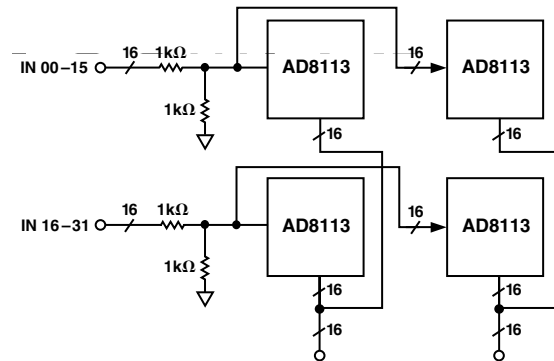
Figure 11. 32 \times 32 Audio Crosspoint Array Using Four AD8113s
