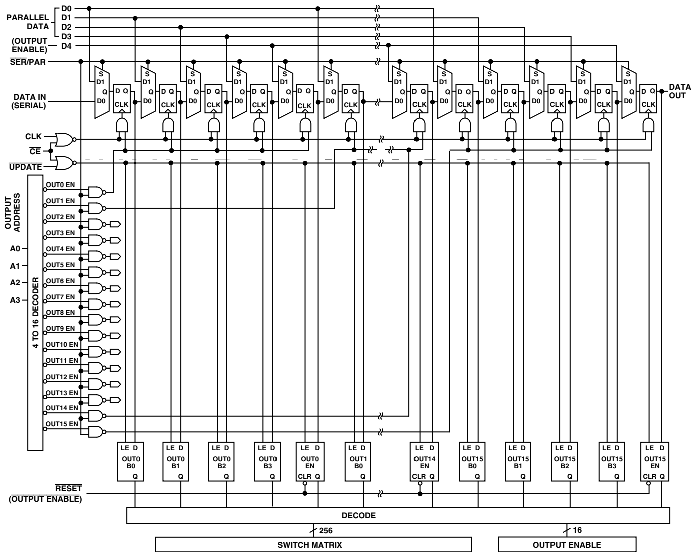
Figure 4. Logic Diagram
