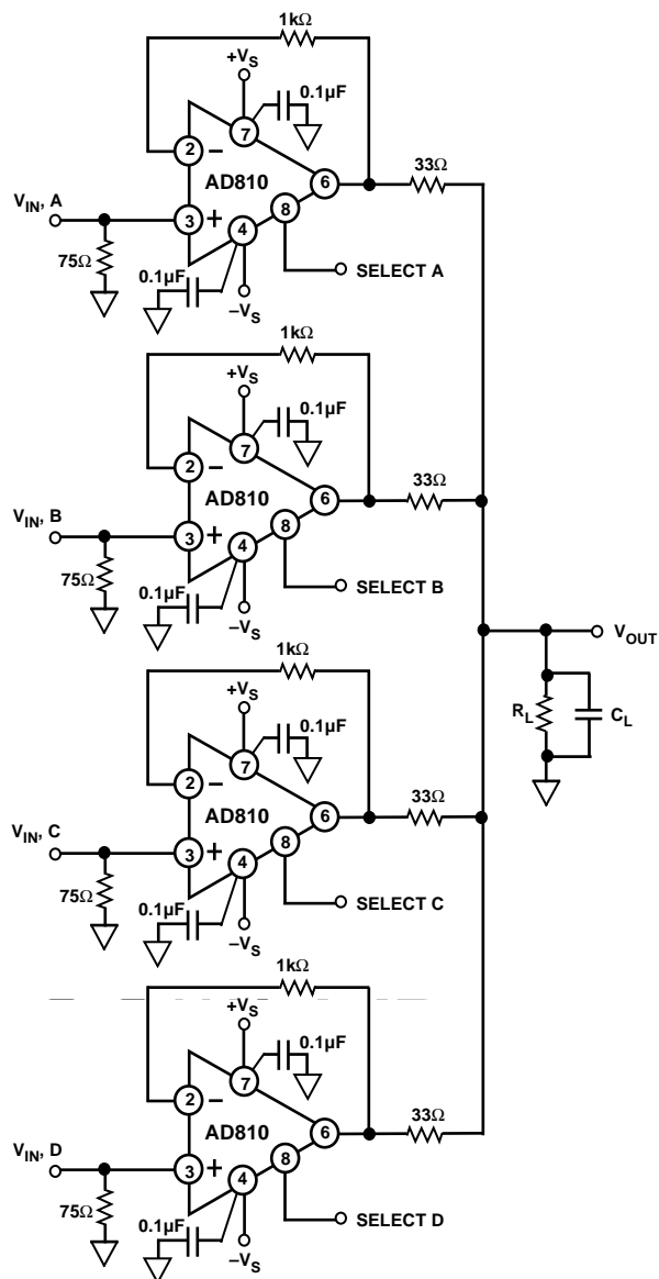
Figure 58. A 4:1 Multiplexer Driving a High Impedance
