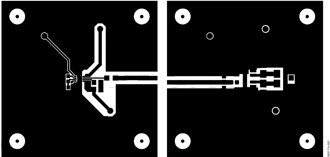
Figure 73. CSP Evaluation Board Artwork
