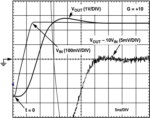
Figure 21. 0.1% Short-Term Settling Time
