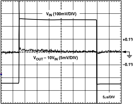
Figure 18. Long-Term Settling Time
