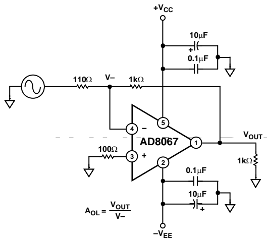
Figure 35. Open-Loop Gain Test Circuit
