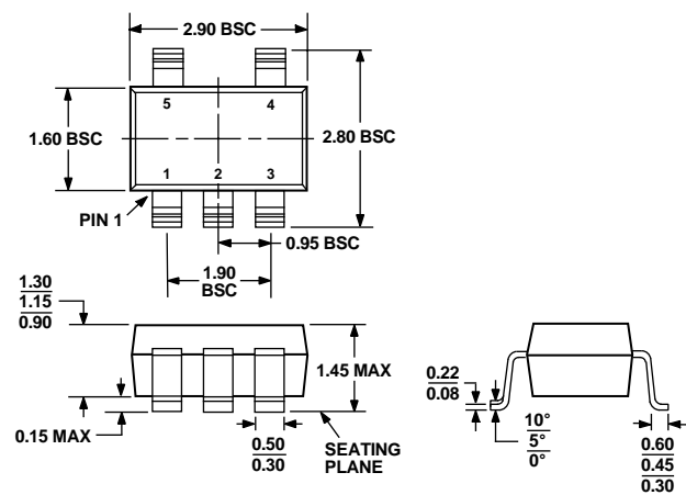
COMPLIANT TO JEDEC STANDARDS MO-178-AA Figure 61. 5-Lead Small Outline Transistor Package [SOT-23] (RT-5) Dimensions shown in millimeters
