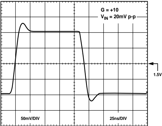
Figure 16. Small Signal Transient Response 5 V Supply
