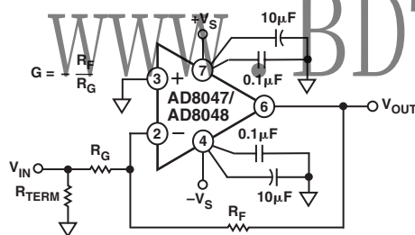
Figure 4. Inverting Operation
