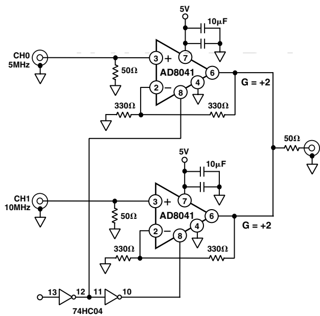
Figure 7. 2:1 Multiplexer
