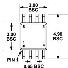
Figure 43. 8-Lead Standard Small Outline Package [SOIC_N] Narrow Body (R-8)—Dimensions shown in millimeters and (inches)
