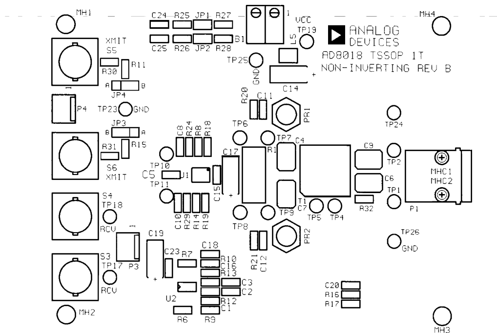
Figure 14. Silk Screen—Primary Side
