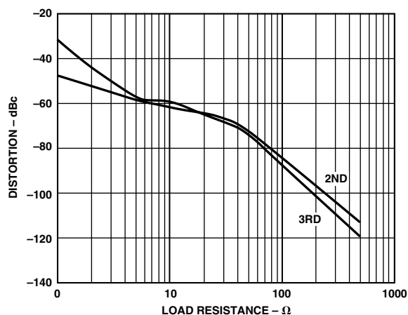
TPC 11. Distortion vs. R_L , V_S = \pm 6V , G = +2 , V_{OUT} = 2V\text{ p-p} , f = 1\text{ MHz}
