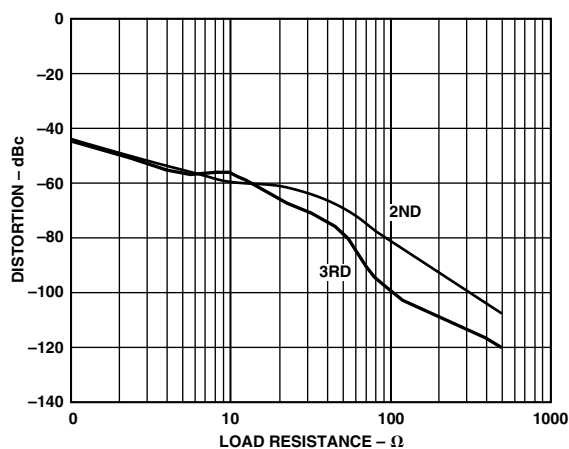
TPC 14. Distortion vs. R_L , V_S = \pm 2.5V , G = +2 , V_{OUT} = 2V\text{ p-p} , f = 1\text{ MHz}
