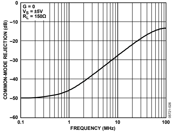
Figure 24. Common-Mode Rejection vs. Frequency
