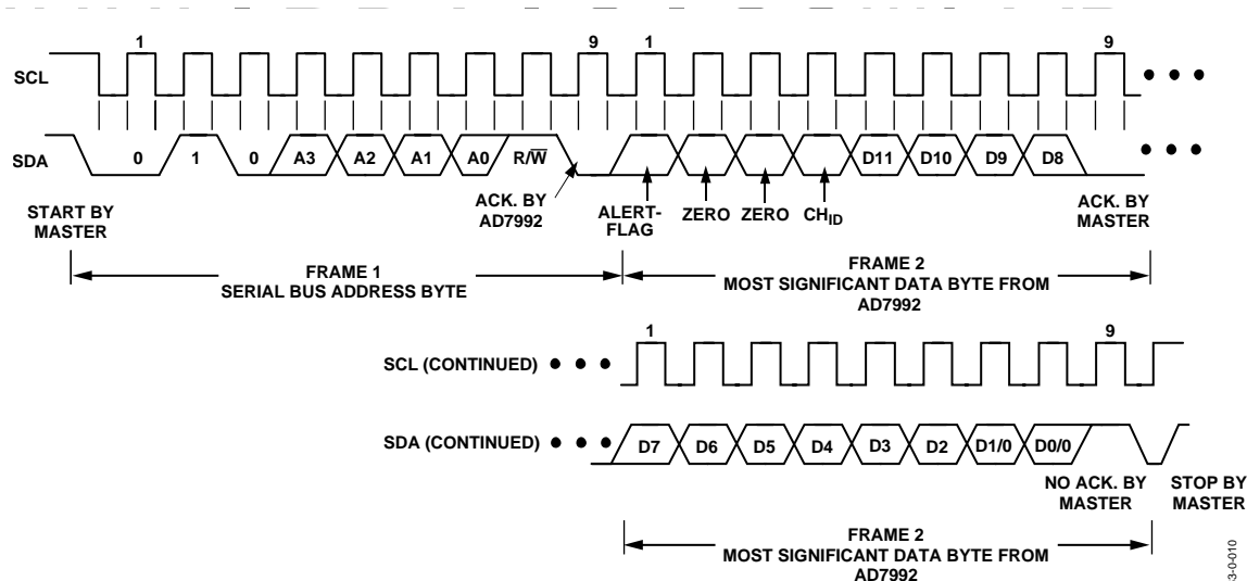
Figure 29. Reading Two Bytes of Data from the Conversion Result Register
