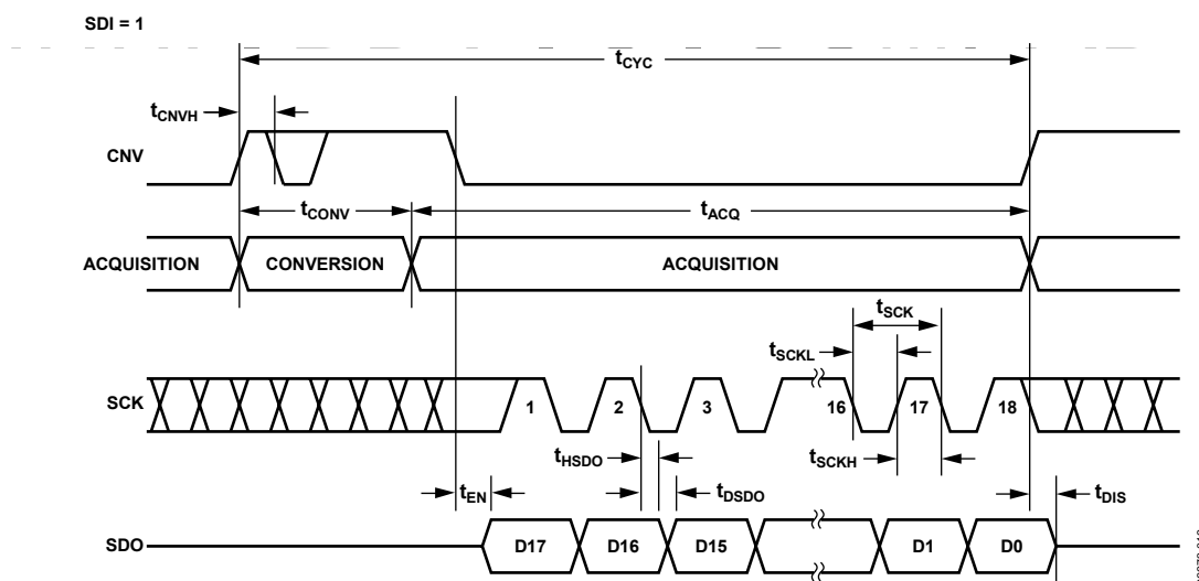
Figure 29. \overline{\text{CS}} Mode, 3-Wire Without Busy Indicator Serial Interface Timing (SDI High)
