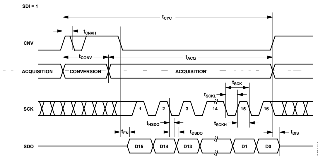
Figure 27. \overline{\text{CS}} Mode, 3-Wire Without Busy Indicator Serial Interface Timing (SDI High)
