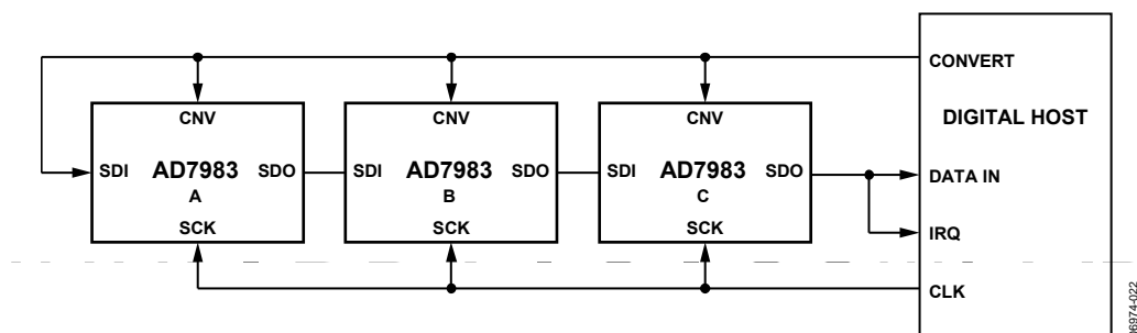
Figure 36. Chain Mode with Busy Indicator Connection Diagram
