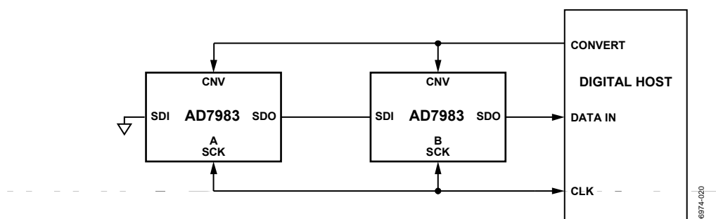
Figure 34. Chain Mode Without Busy Indicator Connection Diagram
