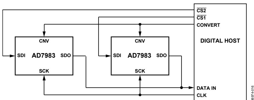
Figure 30. \overline{\text{CS}} Mode, 4-Wire Without Busy-Indicator Connection Diagram
