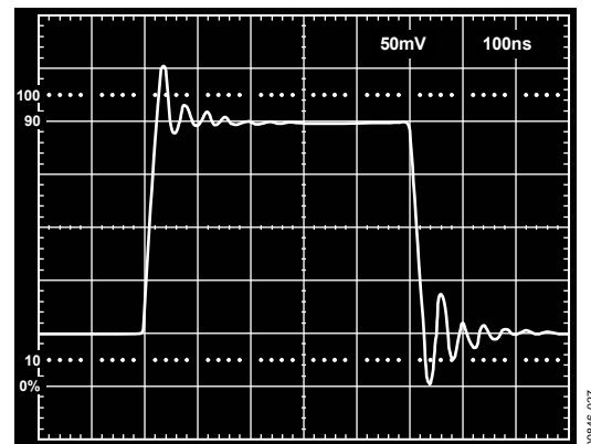
Figure 27. Follower Small-Signal Pulse Response
