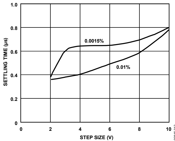
Figure 12. Settling Time vs. Step Size ( \pm )
