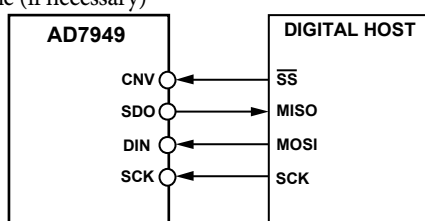
Figure 33. Connection Diagram for the AD7949 Without a Busy Indicator
