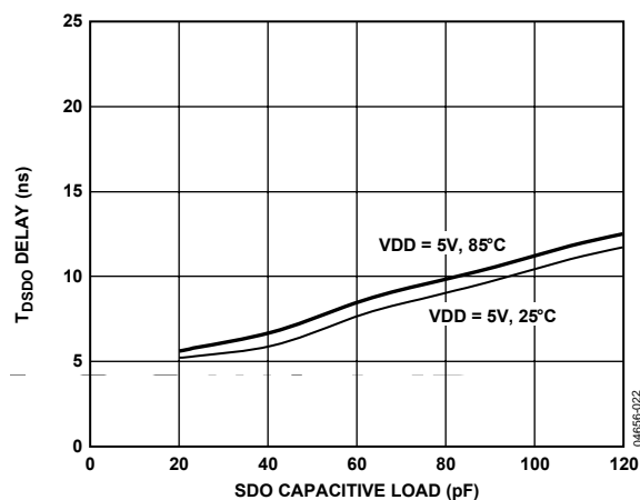
Figure 22. t_{DSDO} Delay vs. Capacitance Load and Supply
