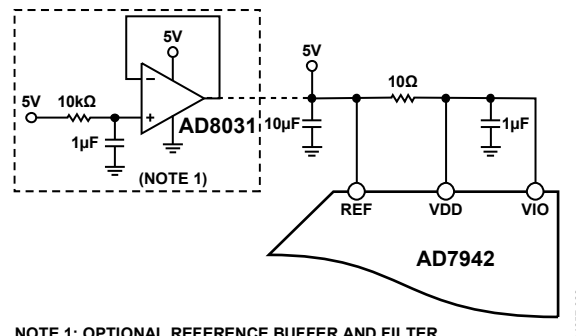
Figure 29. Example of Application Circuit
