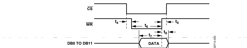
Figure 36. AD7933/AD7934 Parallel Interface—Write Cycle Timing for Word Mode Operation ( \overline{W/B} = 1 )
