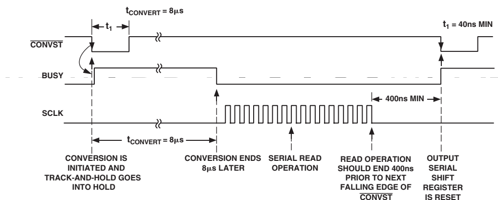
Figure 2. Mode 1 Timing Operation Diagram for High Sampling Performance
