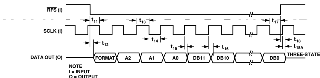
Figure 3. Serial Mode Read Operation
