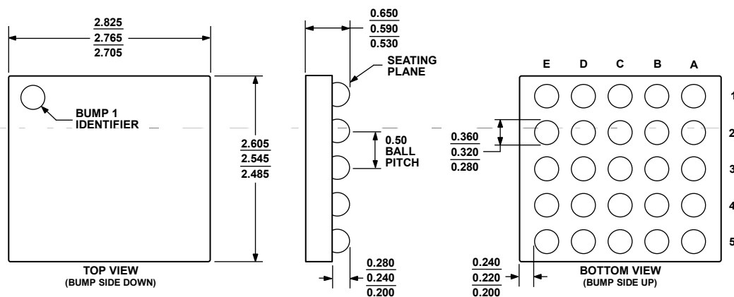
Figure 50. 25-Ball Wafer Level Chip Scale Package [WLCSP]
