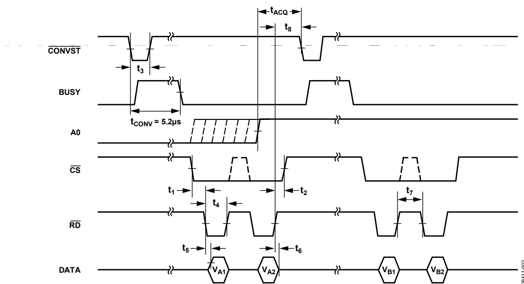
Figure 2. Timing Diagram
