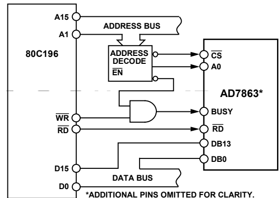
Figure 23. AD7863-80C196 Interface
