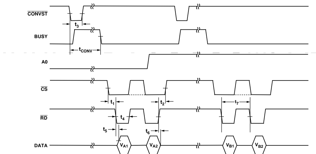
Figure 1. Timing Diagram
