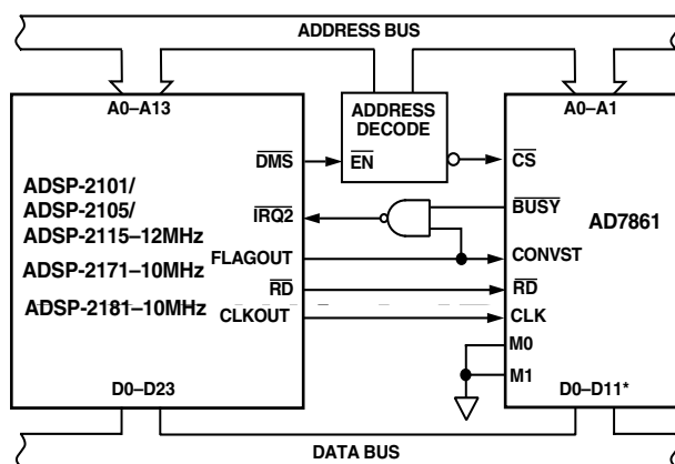
Figure 5. ADI Digital Signal Processor/Microcomputer Interface
