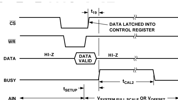
Figure 34. Timing Diagram for System Gain or System Offset Calibration
