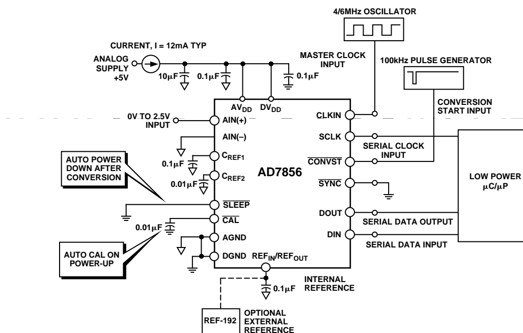
Figure 21. Typical Low Power Circuit
