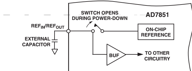
Figure 25. On-Chip Reference During Power-Down
