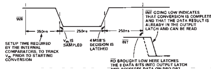
Figure 3. Operating Sequence (WR-RD Mode)
