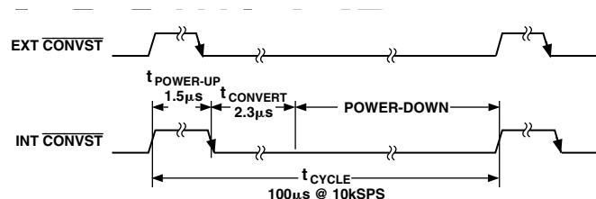
Figure 9. Automatic Power-Down
