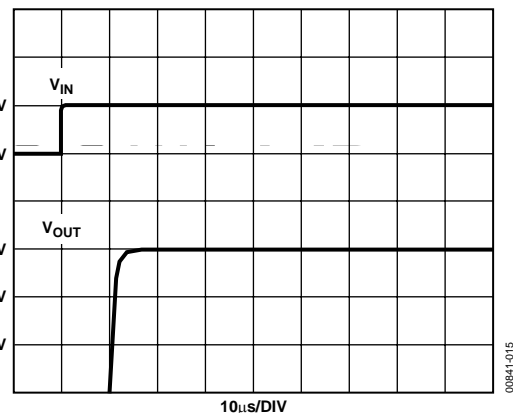
Figure 15. Turn-On Settling Time Performance
