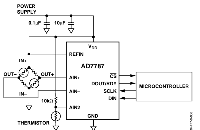
Figure 12. Basic Connection Diagram
