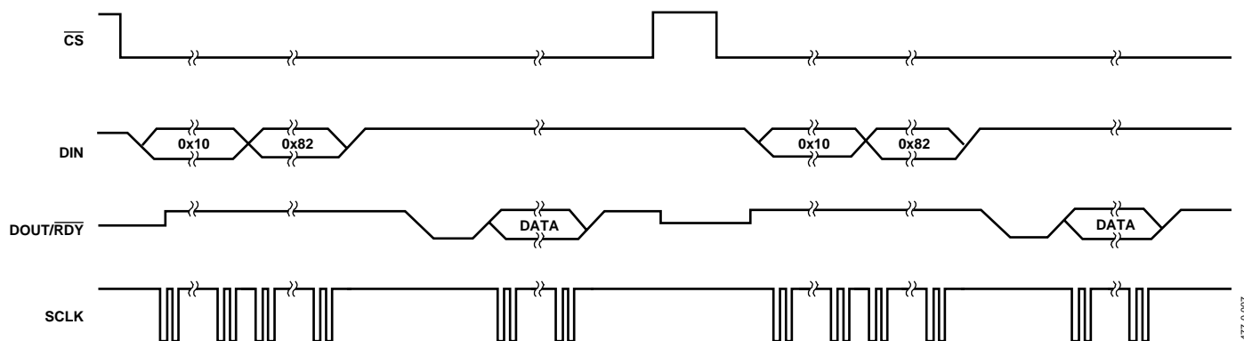
Figure 13. Single Conversion
