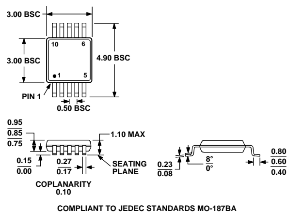
Figure 17. 10-Lead Mini Small Outline Package [MSOP] (RM-10) Dimensions shown in millimeters
