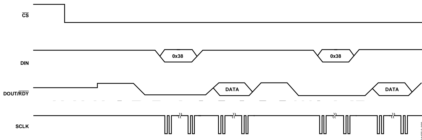
Figure 14. Continuous Conversion
