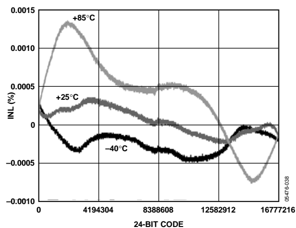
Figure 22. 24-Bit INL, Low Power Mode
