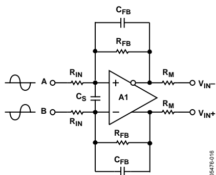
Figure 31. Differential Amplifier Configuration
