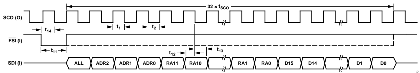
Figure 3. Register Write
