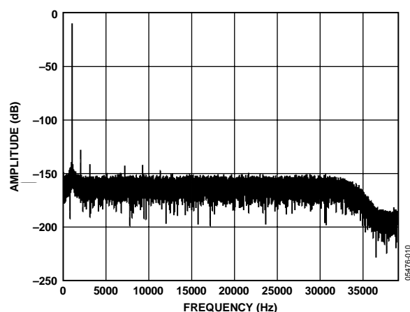
Figure 10. Low Power FFT, 1 kHz, -0.6 dB Input Tone, 256 \times Decimation
