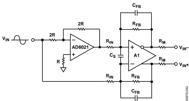
Figure 27. Single-Ended-to-Differential Conversion
