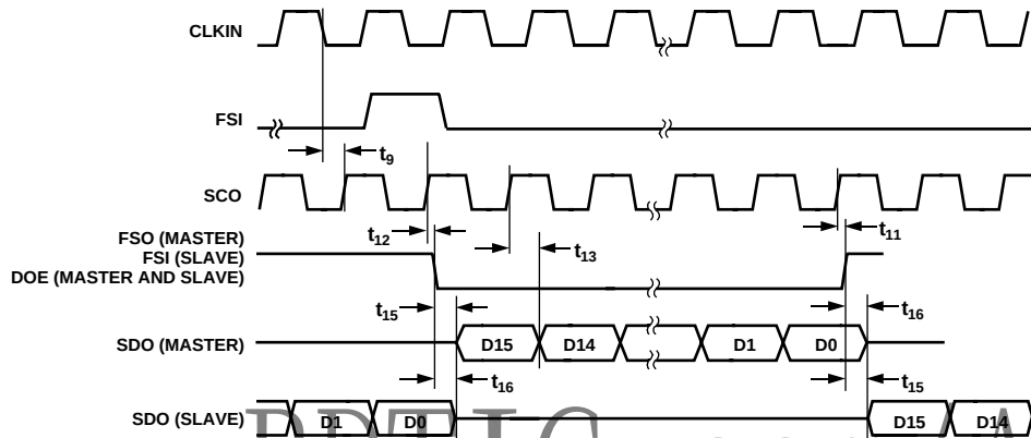
Figure 46. Serial Mode 1 Timing for Two-Channel Multiplexed Operation
