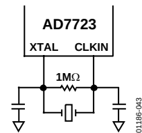
Figure 43. Crystal Oscillator Connection
