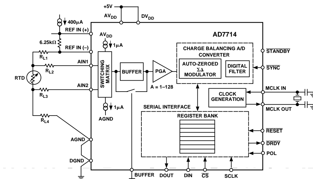
Figure 14. RTD Measurement Using the AD7714
