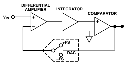
Figure 5. Basic Charge-Balancing ADC
