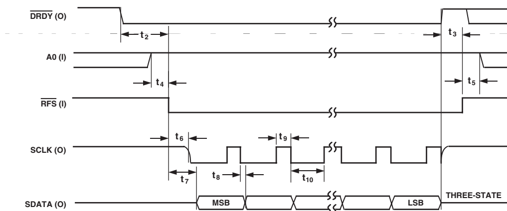
Figure 10. Self-Clocking Mode, Output Data Read Operation
