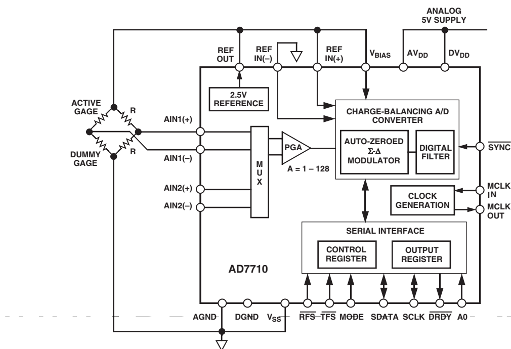
Figure 19. Strain-Gage Application with the AD7710
