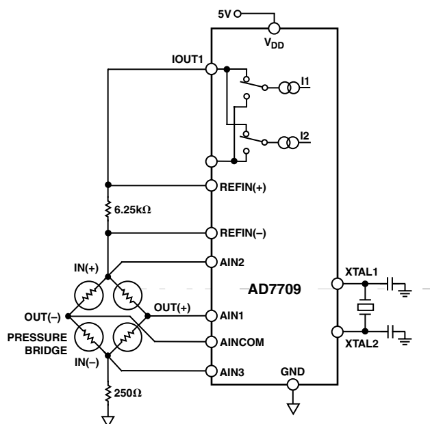
Figure 19. Temperature-Compensating a Pressure Transducer
